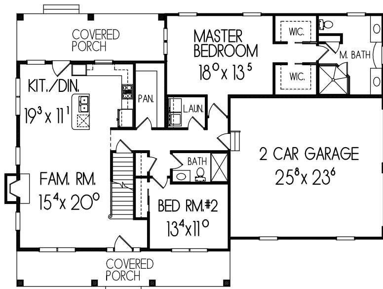
FIRST FLOOR PLAN 2-BEDROOM
