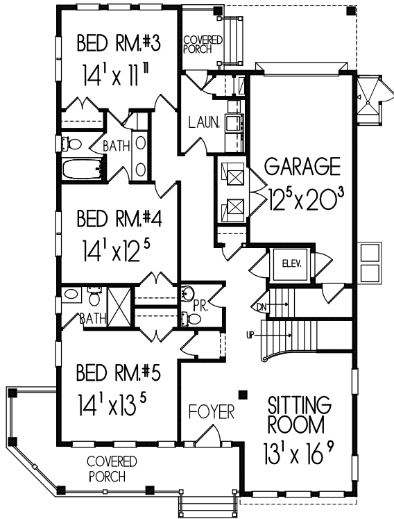
FIRST FLOOR PLAN 3-BEDROOM
